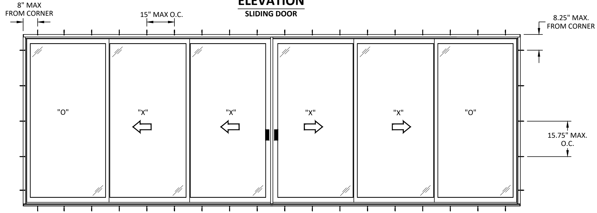
ANCHOR LAYOUT SLIDING DOOR STRAP ANCHOR
